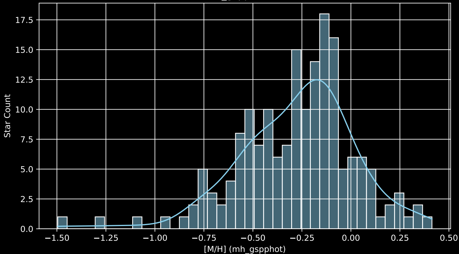
APOGEE DR17 Field: [194+36_MGA [M/H] (mh_gspphot) (n= 174)
