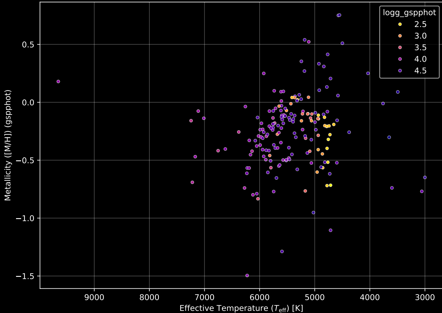
APOGEE DR17 Field: [194+36_MGA] Stellar Population Parameters (n= 179)
