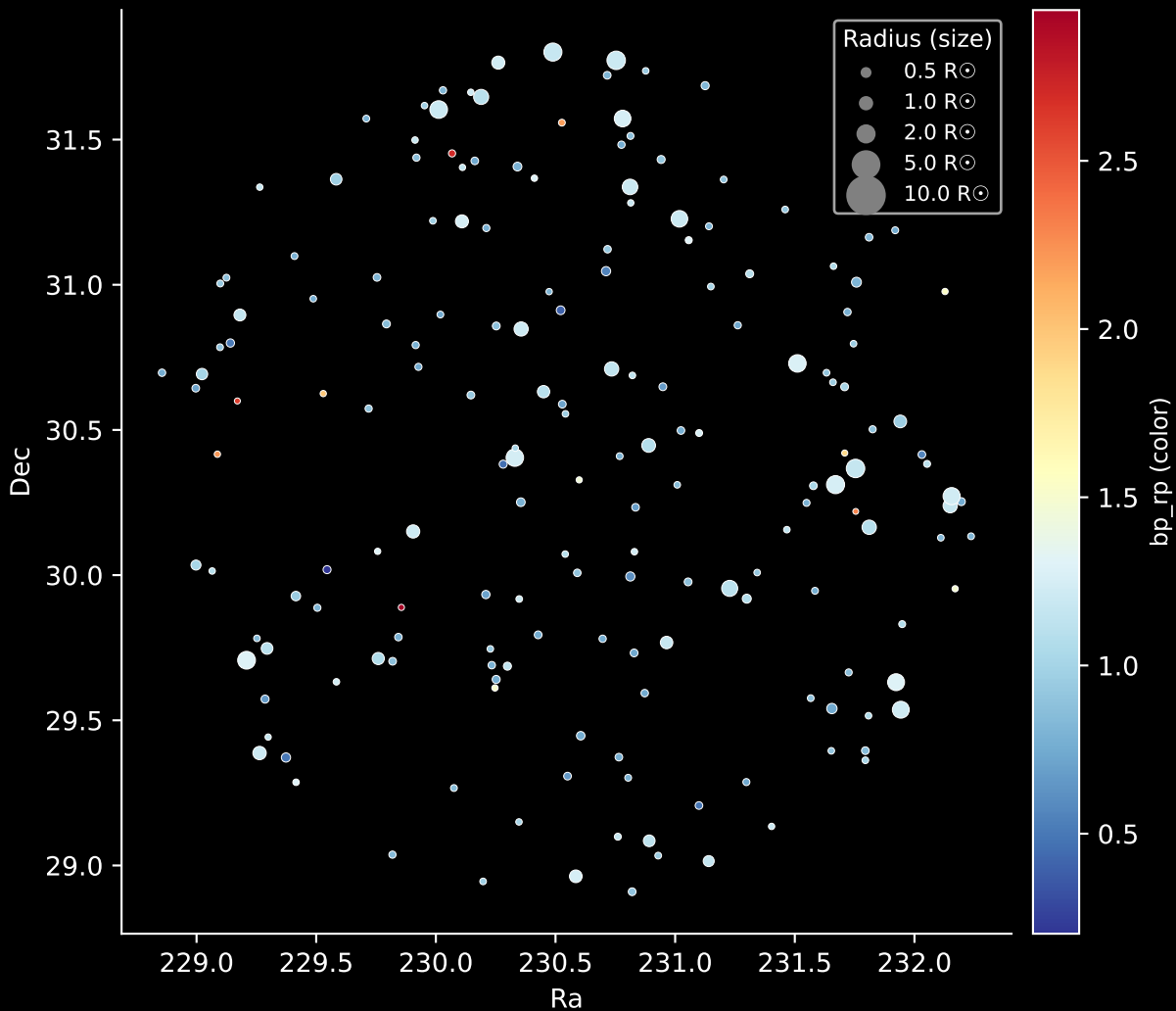
APOGEE DR17 Field: [194+36_MGA] Stars: 179
