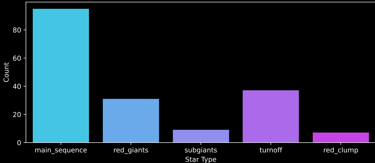
APOGEE DR17 Field: [194+36_MGA] Count plot of Star Type
