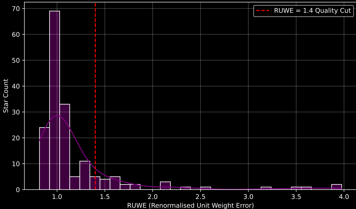
GAPOGEE DR17 Field [194+36_MGA] RUWE Distribution (n= 170)
