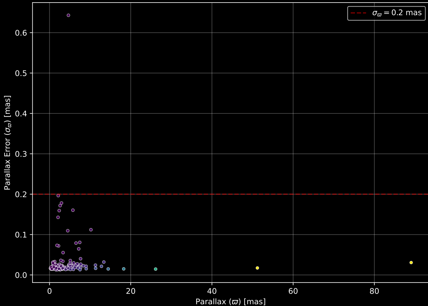
APOGEE DR17 Field: [194+36_MGA] Parallax Quality (n= 179)
