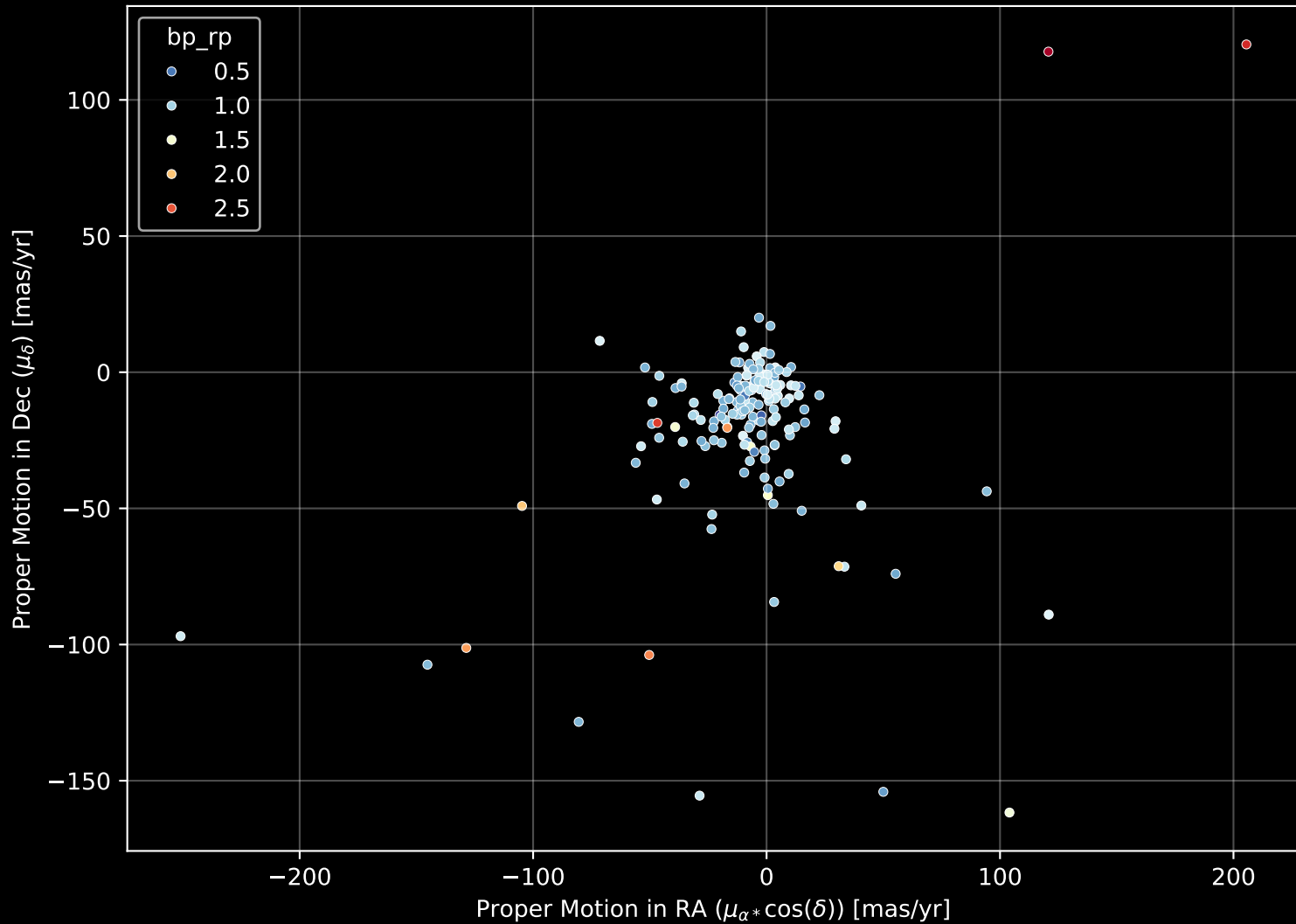
APOGEE DR17 Field: [194+36_MGA] Proper Motion Diagram (n= 179)
